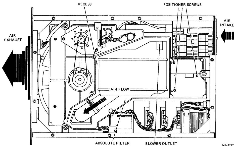
Figure PM-2 RK05J Disk Drive (Bottom View)
