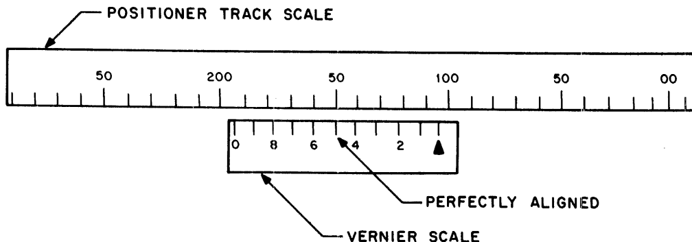
Figure F-1 How to Read a Vernier
