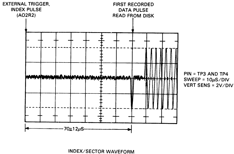
Figure F-2 Index/Sector Waveform
