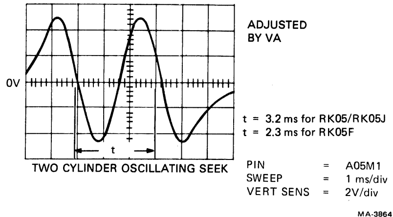
Figure D-3 Velocity Amplitude Waveform
