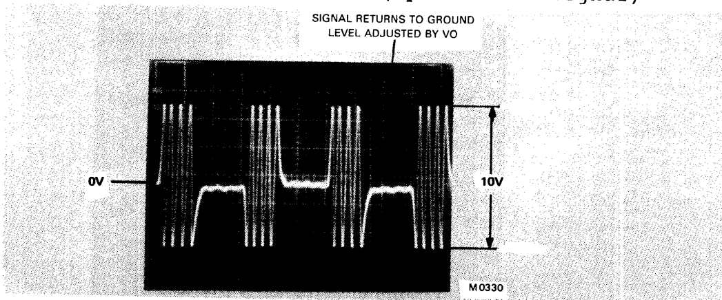
(b) Incorrect Waveform (Signal Not Symmetrical About Ground) Figure D-1 Sine Amplitude/Offset and Velocity Offset Waveform
